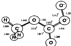
(g) \text{CH}_3\text{OC}(\text{O})\text{O}_2
